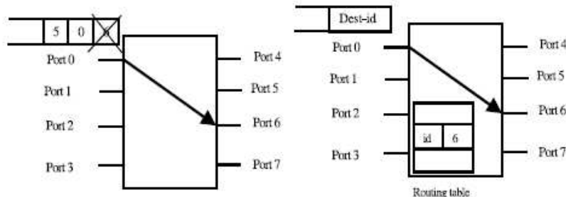
Figure 6: Source-path routing vs. table-based routing.
