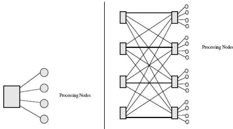
Figure 8: Quaternary fat tree of dimension 1 (left) and Elite switch of Quadrics networks (right).
