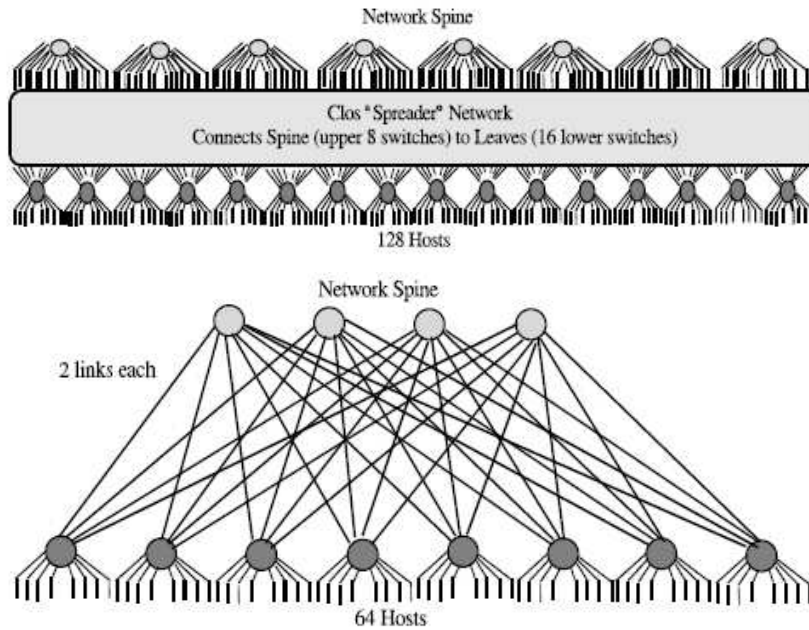
Figure 7: A 128-host Clos network using 16-port Myrinet switch (upper) and a 64-host Clos network using 16-port Myrinet switch (each line represents two links).
